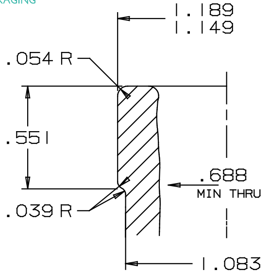
FINISH DETAIL SCALE 2 x 1
